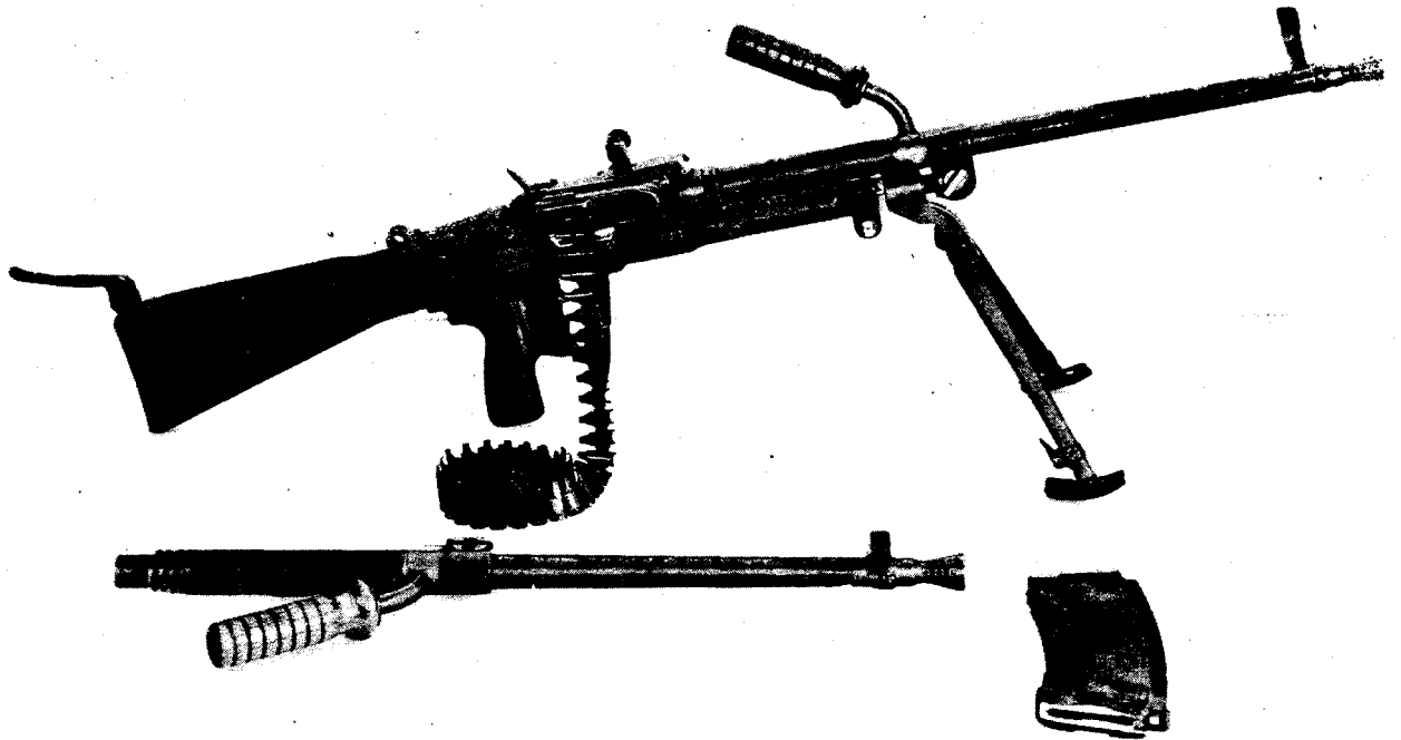
Figure 44. Czechoslovak 7.62-mm Light Machinegun Model 52.
